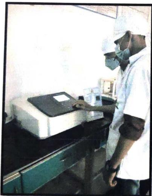
UV-1800 Spectrophotometer
